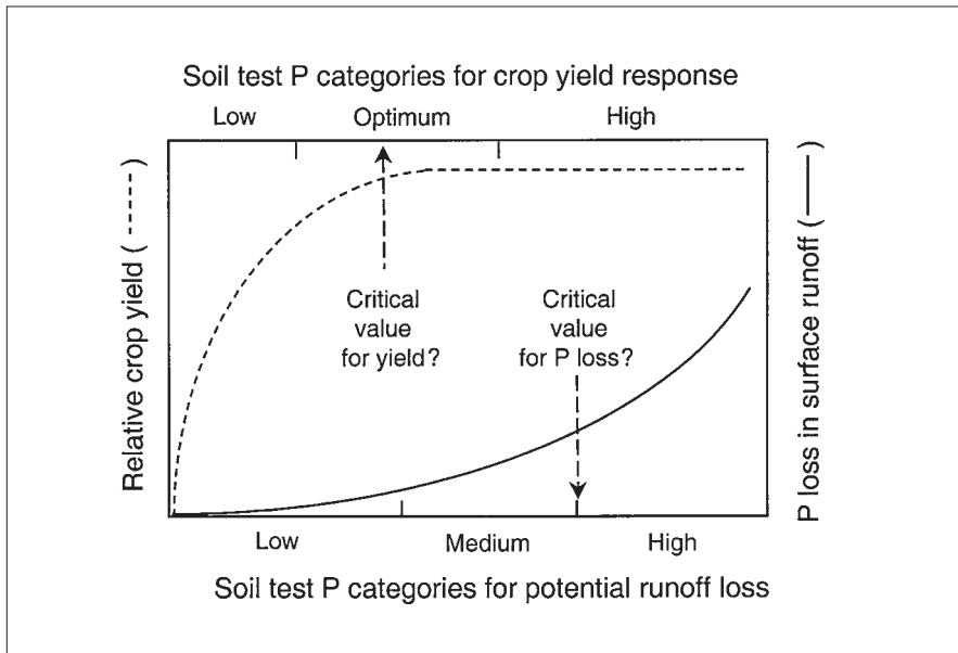
Figure 34-14. As soil P increases, so does crop yield and the potential for P loss in surface runoff. The interval between the critical soil P value for yield and runoff P is important for P management.
