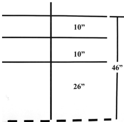
b. Three-wire horse fence.
