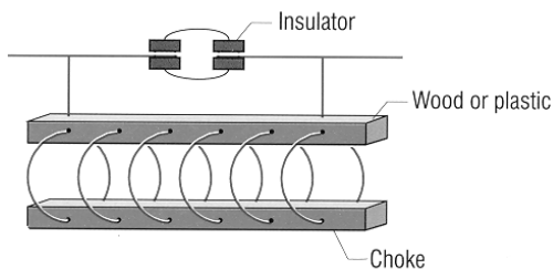
Figure 11. Induction coil/lighting choke.
