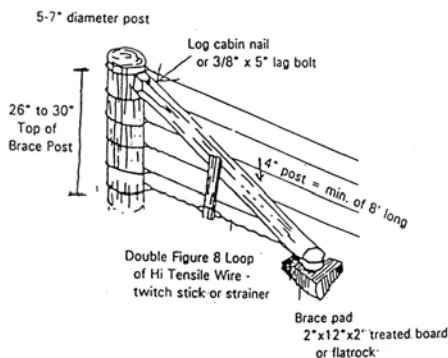
a. Figure 4 end post. Figures 9a and b. End post assemblies.
