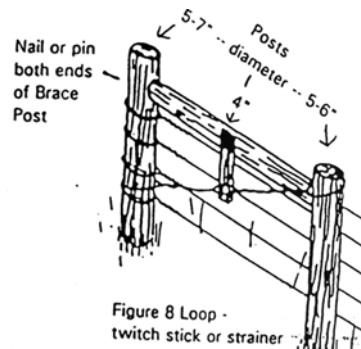
b. H brace end post.
