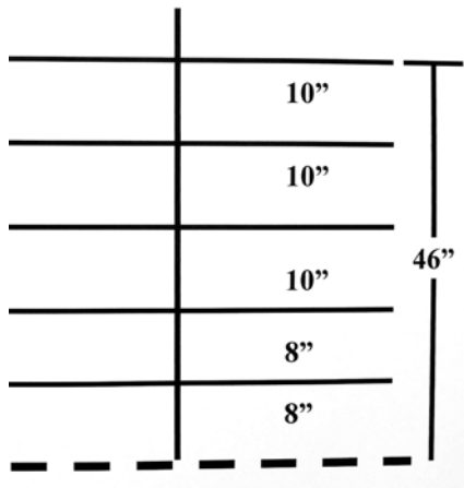
a. Five-wire cattle fence.
