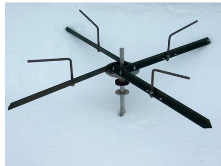
Figure 10. Pay out spinner.
