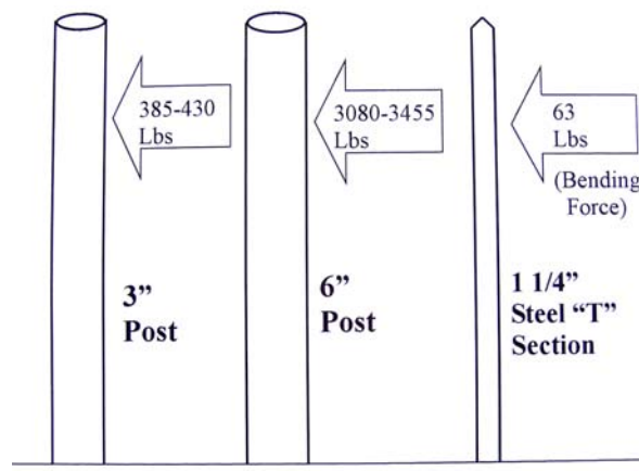
Figure 3. Fence post strength (breaking force required for wood post).
