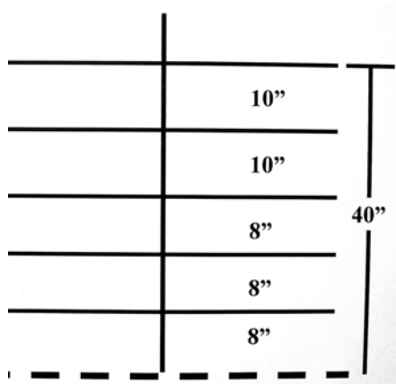
c. Five-wire sheep/goat fence.
