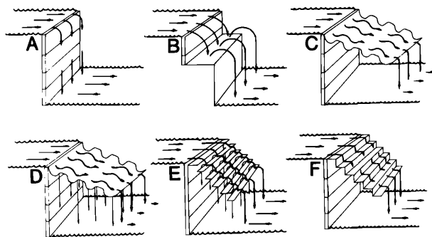
Fig. 1. Diagrams of gravity aerators. A, Simple weir (Haskell et al. 1960; Chesness and Stephens 1971); B, splashboard (Haskell et al. 1960; Chesness and Stephens 1971); C, inclined corrugated sheet (Chesness and Stephens 1971); D, inclined corrugated sheet with holes (Chesness and Stephens 1971); E, lattice aerator (Chesness and Stephens 1971); and F, cascade aerator (Tebbutt 1972).
