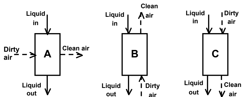
Figure 1. Flow configurations for operating scrubbers: (A) cross, (B) counter-current, and (C) concurrent.
