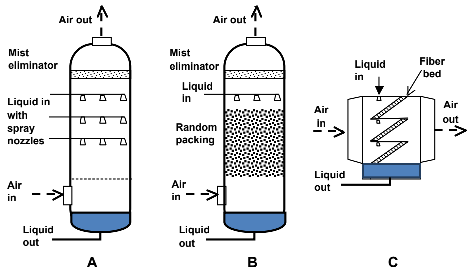
Figure 2. Schematic diagrams of spray scrubber (A) packed bed, (B) and fiber-bed, (C) scrubbers.
